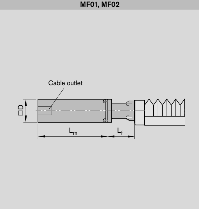
Motor attachment with motor mount and coupling MF01, MF02
